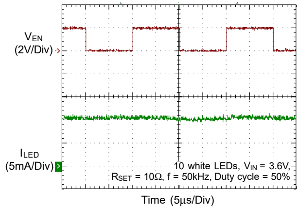
PWM Dimming from EN
