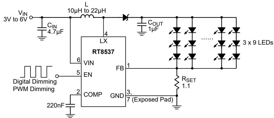
Figure 1. Drive 27 LEDs for Media form Factor Display
