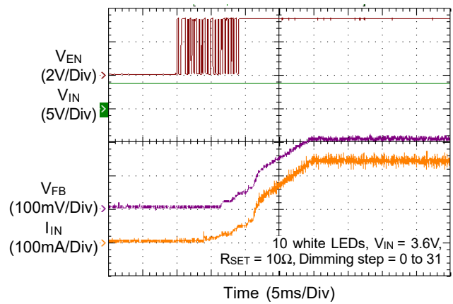
1-Wire Dimming from EN On
