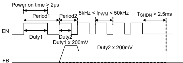
Figure 5. PWM Dimming Control
