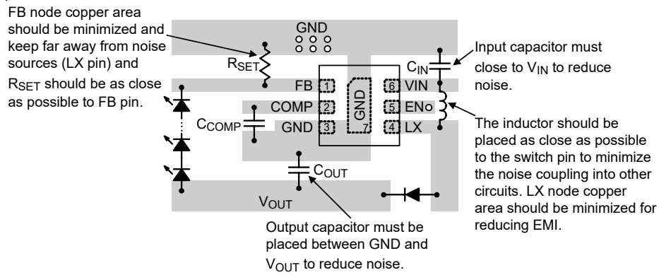
Figure 9. PCB Layout Guide
