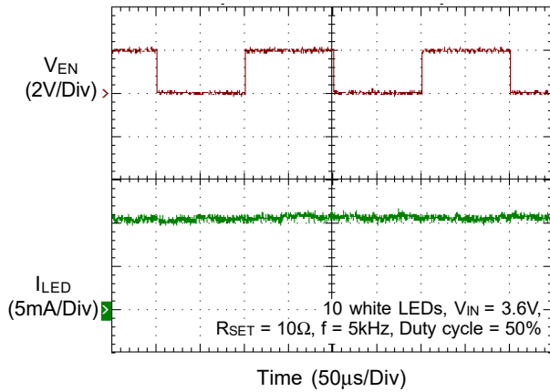
PWM Dimming from EN
