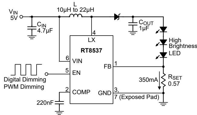
Figure 2. Application Circuit for 3 High Brightness LEDs
