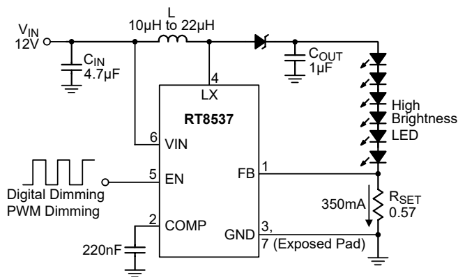
Figure 3. Application Circuit for 6 High Brightness LEDs
